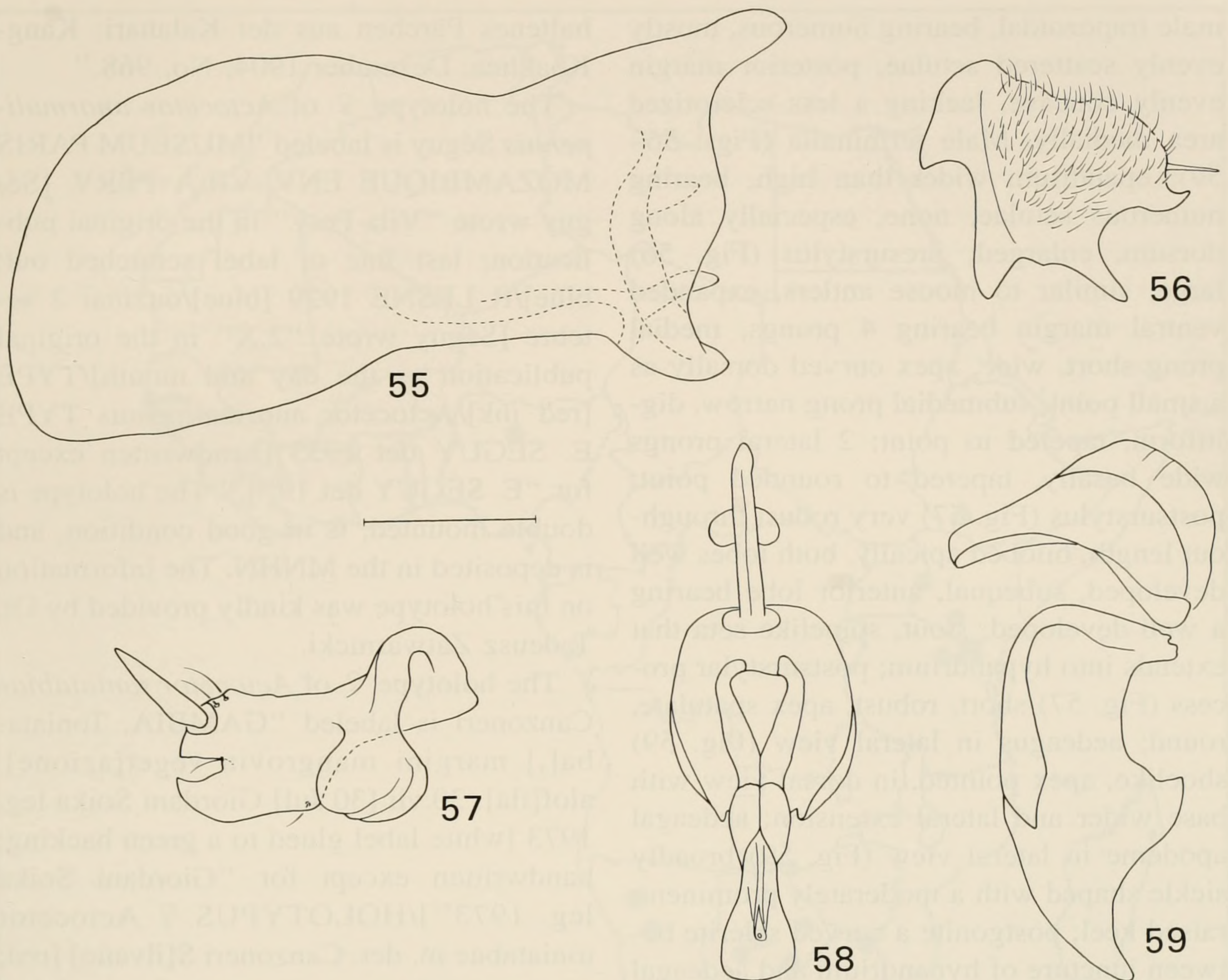
Figs. 55–59. Structures of the male preabdomen and terminalia of Actocetor decemguttatus . 55, Hypandrium, lateral view. 56, Presurstylus, posterior view. 57, Postsurstylus, lateral view. 58, Aedeagus, aedeagal apodeme, dorsal view. 59, Same, lateral view. Scale bar equals 0.1 mm.
